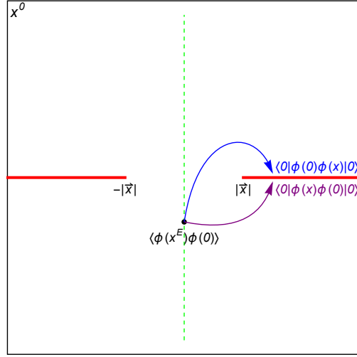
Figure 24: The complex x^0 -plane, with the imaginary x^0 -axis (negative Euclidean time) indicated by the dashed green vertical line. The Wightman functions \langle 0|\phi(x)\phi(0)|0\rangle and \langle 0|\phi(0)\phi(x)|0\rangle are obtained as the analytic continuations of the Euclidean 2-point function \langle \phi(x^E)\phi(0)\rangle above and below the branch cuts x^0 \in (-\infty, -|\vec{x}|] \cup [|\vec{x}|, \infty) respectively.
