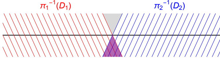
Figure 10: The uplifted patches \pi_1^{-1}(D_1) and \pi_2^{-1}(D_2) generally do not agree along D_1 \cap D_2 . The integrals along the fibers of \pi_1 and \pi_2 must be supplemented by the integration over the interpolating patch, shown in gray (with positive orientation) and purple (with negative orientation).
